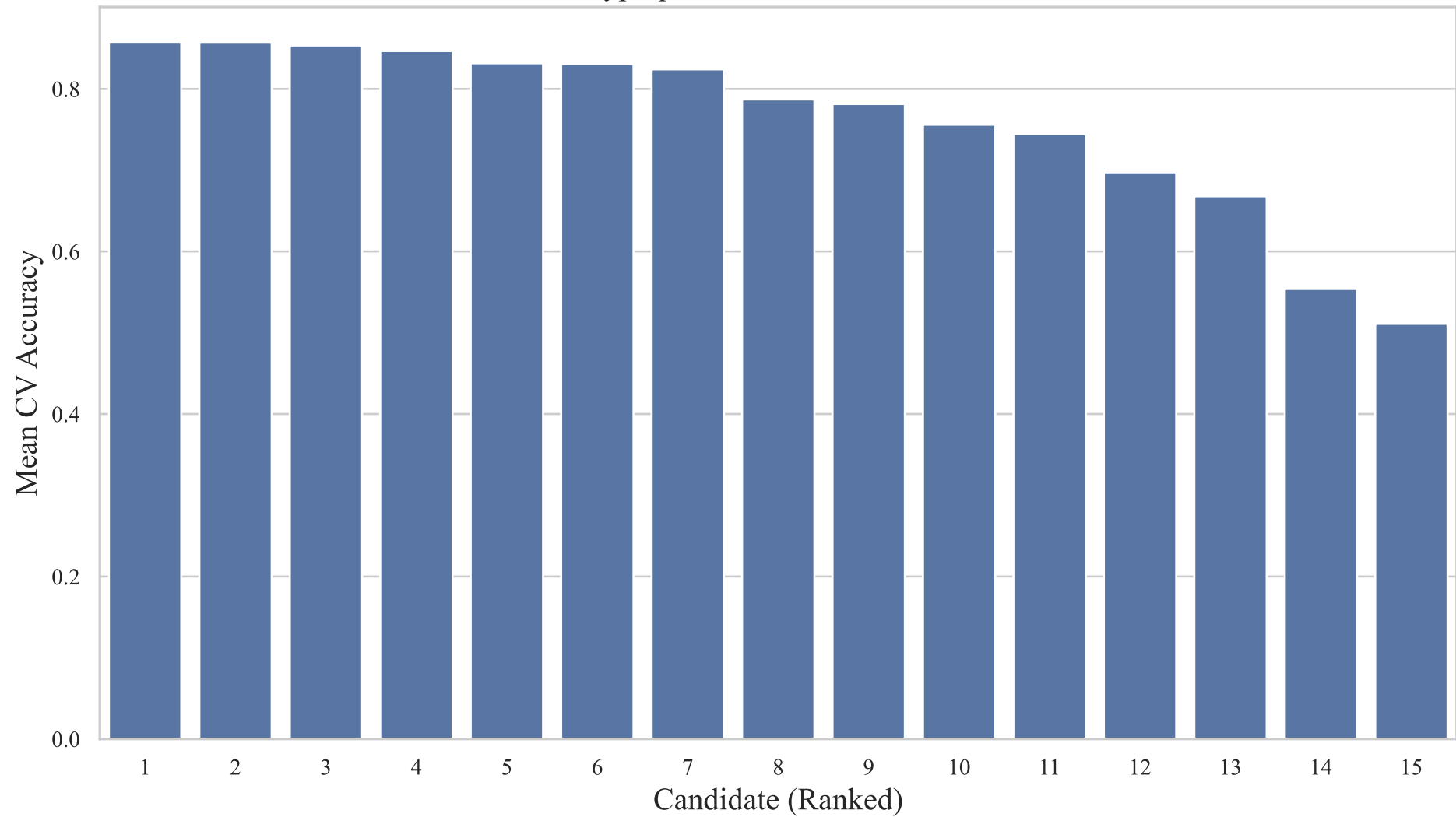
Hyperparameter Search Results
